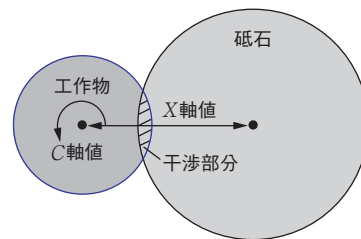
図5 砥石と工作物の位置関係 Geometrical relationship between wheel and workpiece
