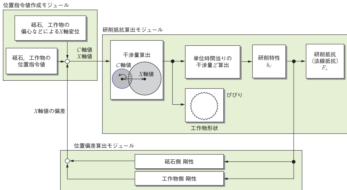
図4 びびりの予測手順 Predicting procedure of chatter
